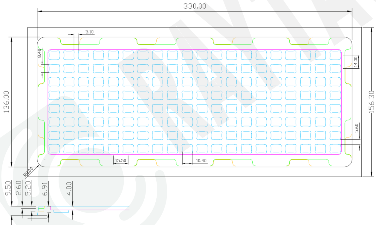
Figure 1: Tray specification with PET marking
