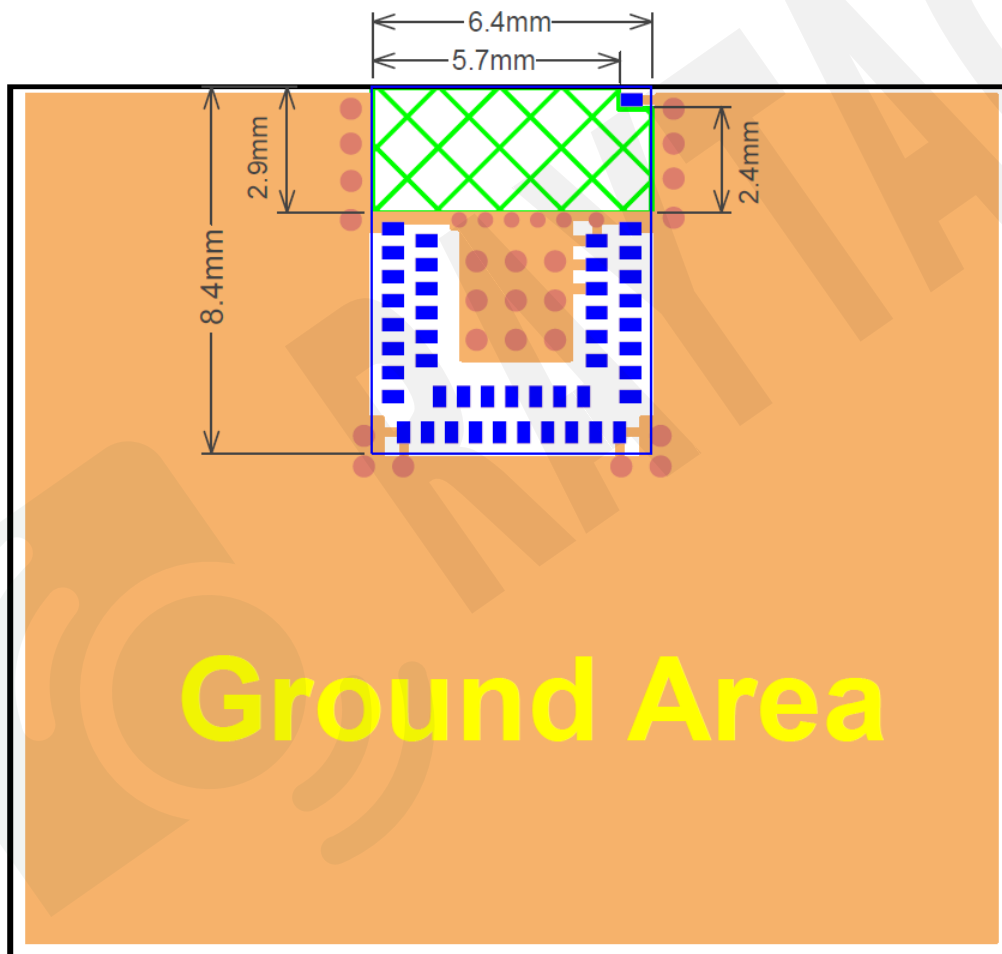
Top View
