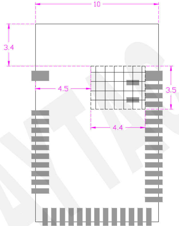
Toplayer no ground pad
